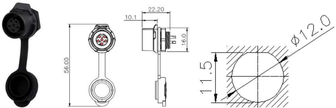
LP-12-J SX-XX-001 Single hole female socket
